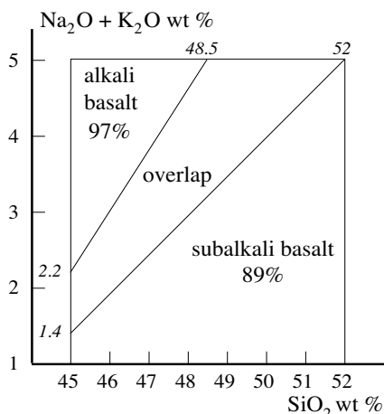
Fig. 2.16. Likelihood of correctly classifying alkali basalt and subalkali basalt using TAS (after Bellieni et al. 1983) assuming equal chances of a basalt being alkali or subalkali.
